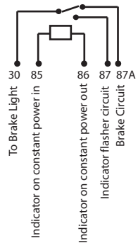
5 Pin Relay Diagram
